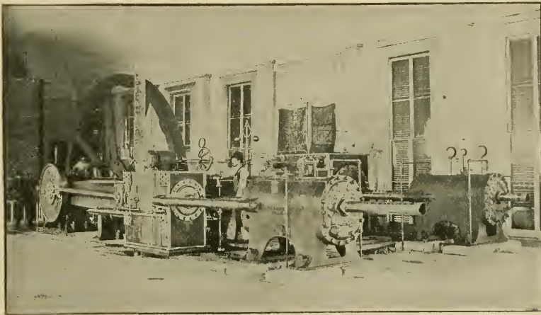
THE POWER PLANT AT JEROME PARK, N. Y. (Ingersoll-Sergeant Duplex Corliss Condensing Air Compressor.)
